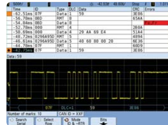
Industry's only real-time hardware-based serial decode for I 2 C, SPI, CAN, LIN, FlexRay, RS232/UART, PS and MIL-STD-1553
