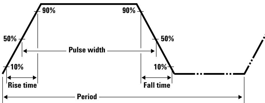
Figure 4. Pulse waveform parameters
