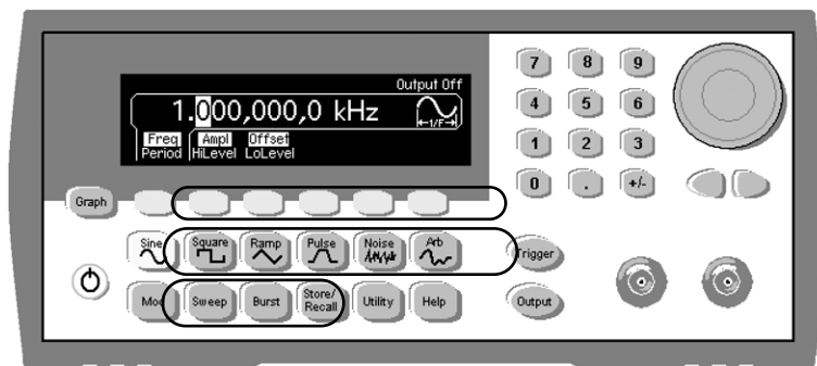
Figure 1. The Agilent 33220A and 33250A function generator user interface groups together common waveforms and provides clearly labeled keys so you can complete simple tasks more easily.
