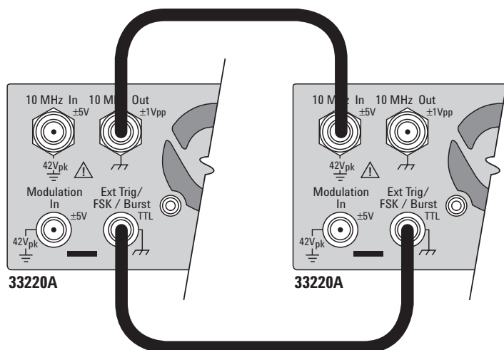
Figure 6. Two externally locked 33220A generators. The generators are using a common clock signal and a common trigger signal.
