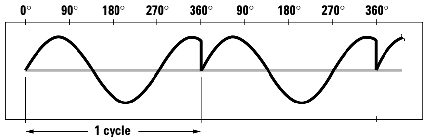
Figure 3. Create arbitrary waveforms as a single period or as integer-multiple periods to avoid discontinuities
