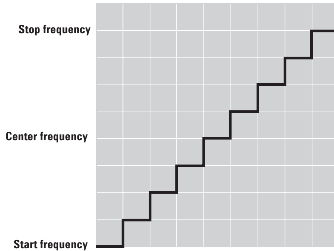
Figure 8. Arbitrary waveform used with FM mode to create a stepped sweep.
