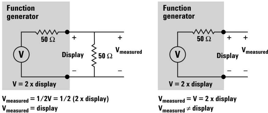
Figure 2. When you add a 50-ohm load to the output of the function generator, as shown in the diagram on the left, the measured and displayed voltage will be the same.
