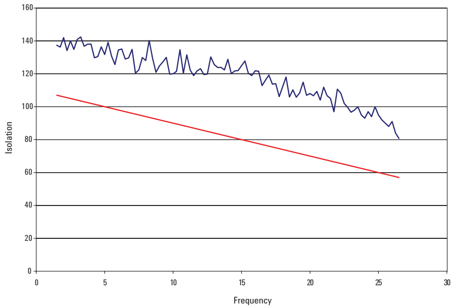
Figure 14. Agilent L7222C isolation versus frequency
