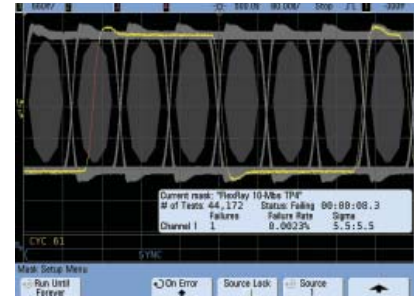
Figure 2: Testing a FlexRay eye-diagram with an imported industry-standard mask.
