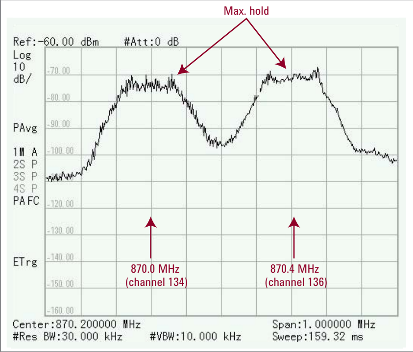
Figure 3. Over-the-air measurement of a GSM 850 downlink transmission using the Agilent N934xC HSA with the trace "Maximum Hold" selected
