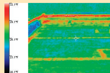
Figure 5. Cool areas on this roof exposure probably indicate moisture buildup. Mark with tape and investigate with core samples.
