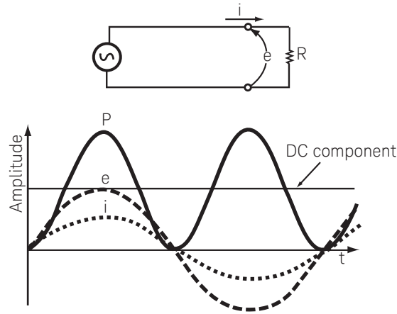
Figure 2-2. The product of voltage and current, P, varies during the sinusoidal cycle.
