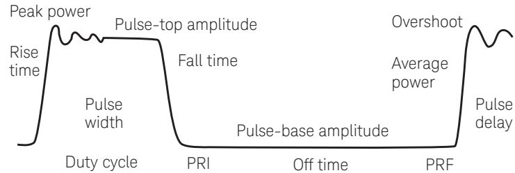
Figure 2-5. Typical envelope of pulsed system with overshoot and pulse ringing, shown with 13 pulse parameters which characterize time and amplitude.
