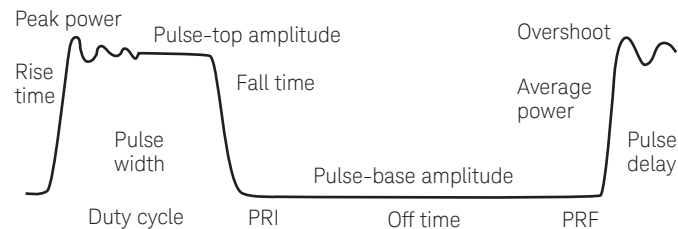
Figure 1-1. Typical envelope of pulsed system with overshoot and pulse ringing, shown with 13 pulse parameters which the Keysight 8990A characterized for time and amplitude.
