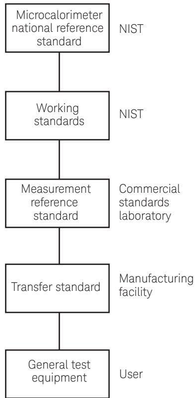
Figure 3-1. The traceability path of power references from the United States National Reference Standard.
