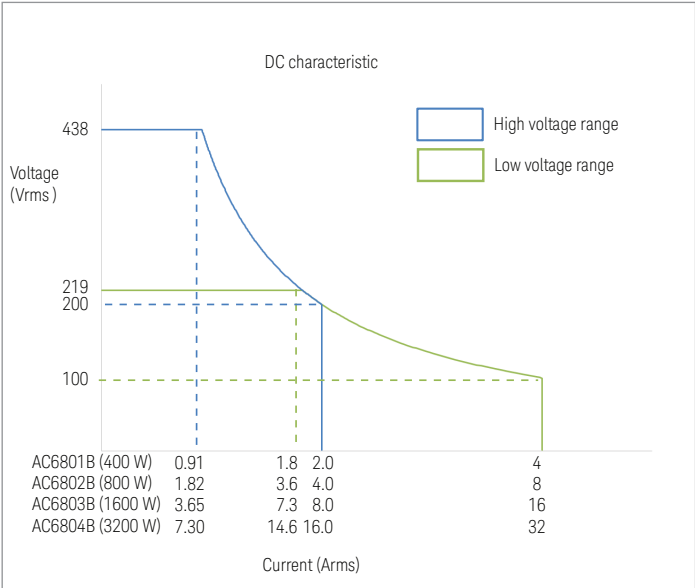
AC6800B steady-state DC output characteristic
