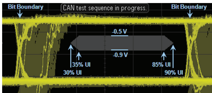
Figure 8. Pass/Fail mask for a 10 meter network operating at 500 kbps
