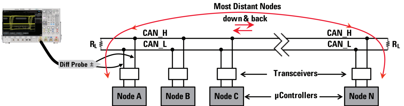
Figure 6. Typical multi-node CAN 2.0 network
