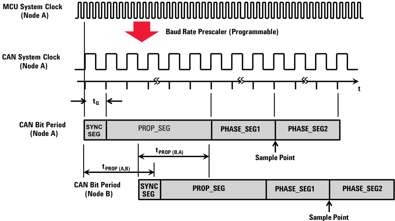
Figure 5. CAN bit-timing diagram for two widely-spaced nodes
