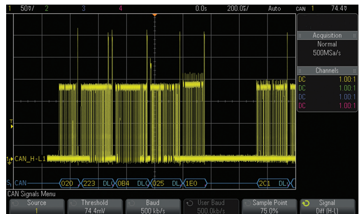
Figure 2. Probing the differential CAN bus to show dominant-bit-high
