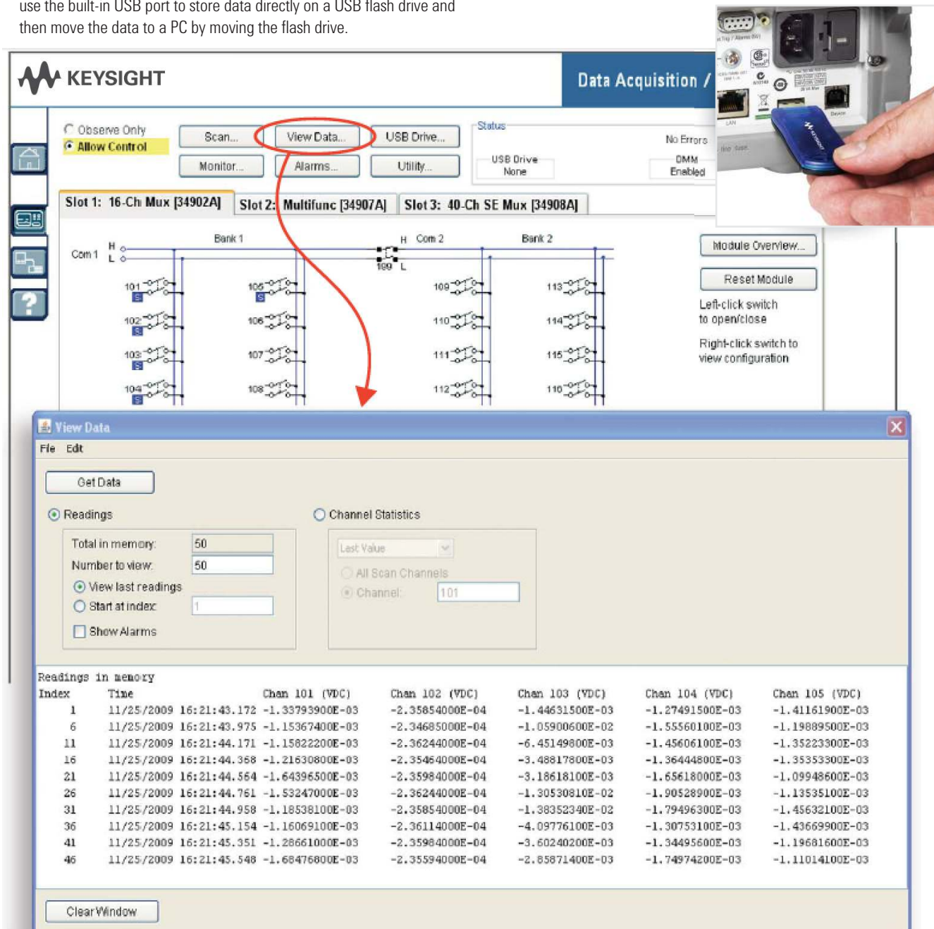
Figure 4: View, copy, and paste measured data or store it directly in CSV format
