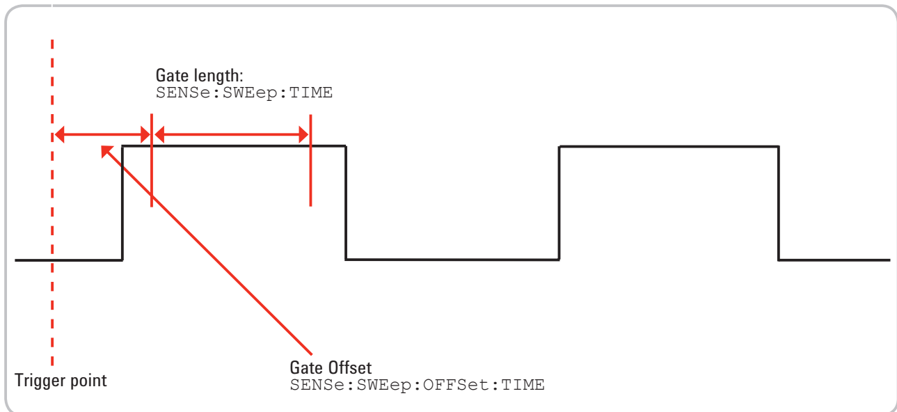
Figure 7. Diagram of a time-gated signal
