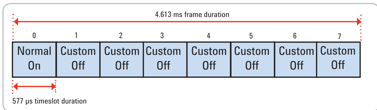
Figure 4. GSM timeslot pattern with timeslot 0 on
