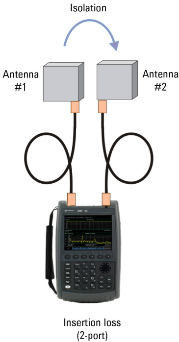
Figure 6b. Configuration for measuring antenna-to-antenna isolation
