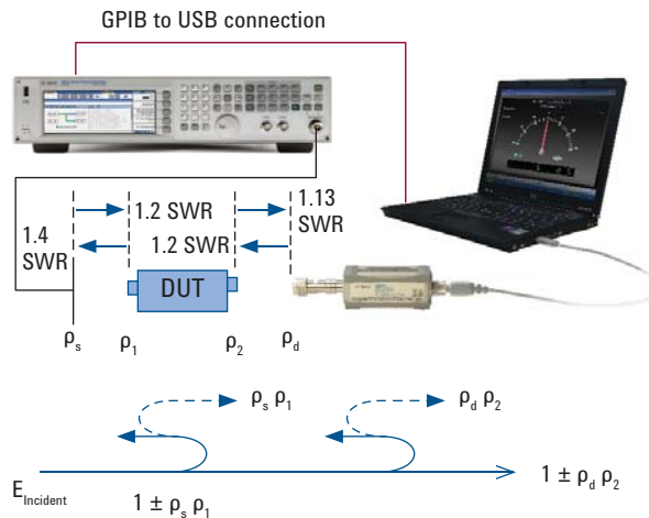
Figure 9. Mismatch uncertainties for measurement (post leveling transmission measurement)
