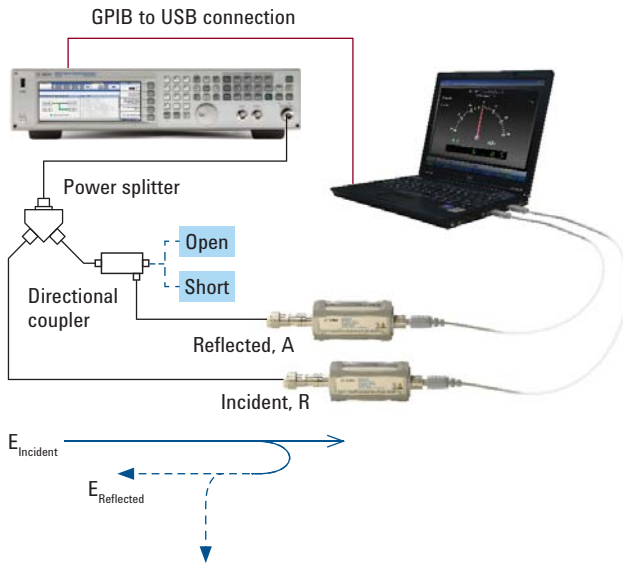
Figure 14. Calibration setup prior to reflection measurement
