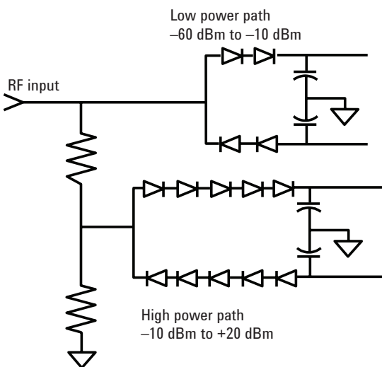
Figure 7. Schematic of a diode-attenuator-diode sensing element
