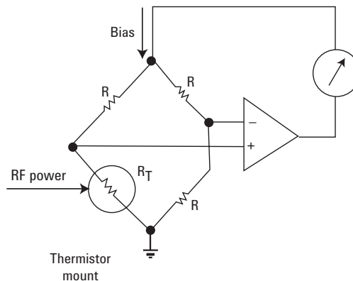
Figure 3. Bridge technique used in thermistor sensor
