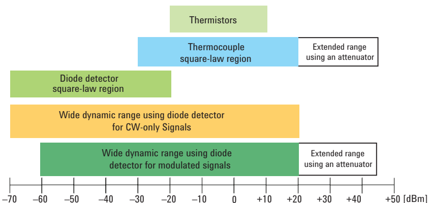
Figure 10. Power range of various sensor types
