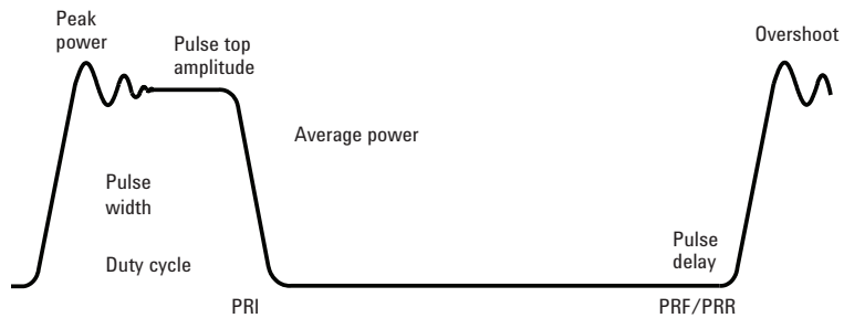
Figure 2. Typical radar pulse characteristics
