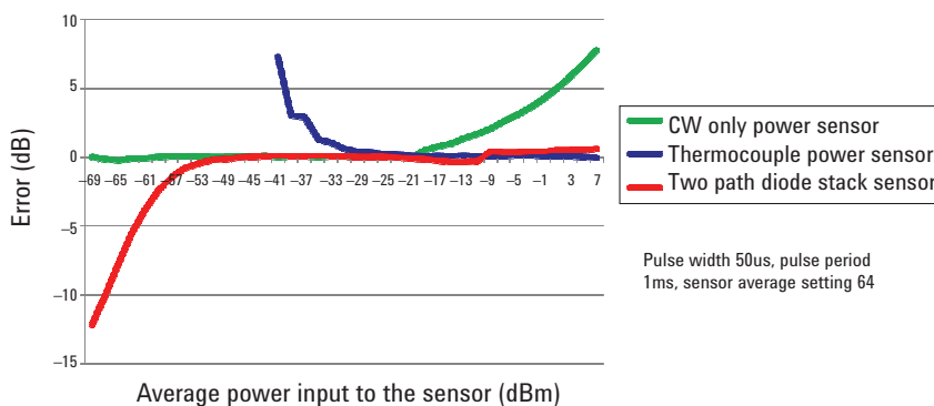
Figure 9. Comparison of three sensor types for pulse power measurement
