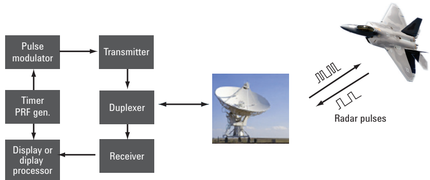
Figure 1. Block diagram of a simple radar system
