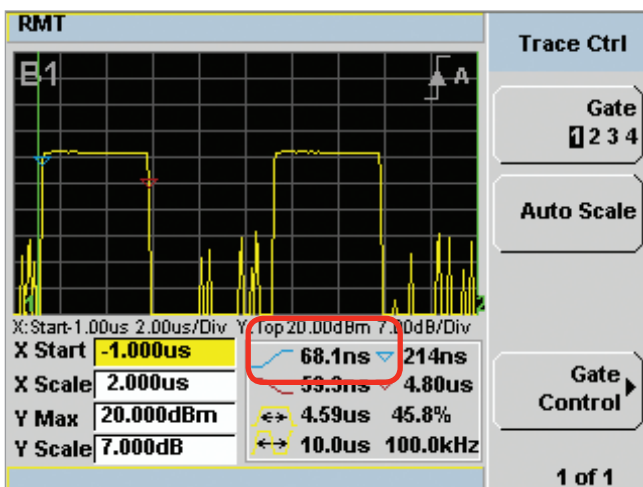
Figure 13. A peak power meter uses continuous sampling and 30 MHz video bandwidth to accurately measure fast rise and fall times.
