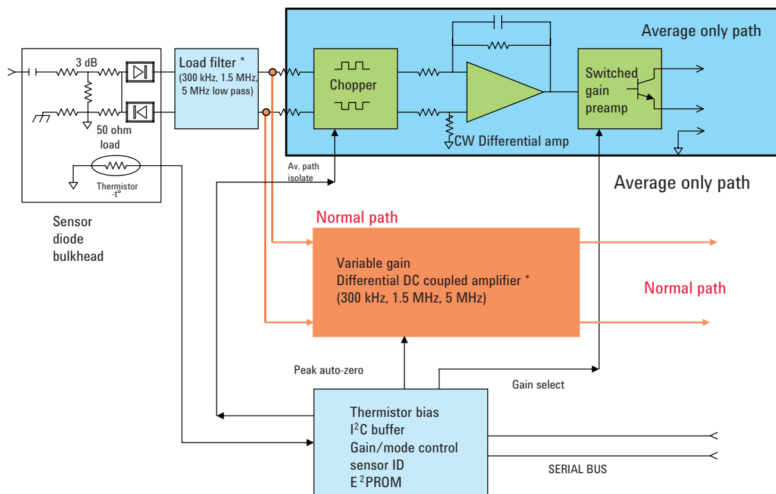
Figure 8. Block diagram of a peak and average sensor showing the parallel amplification paths, one for “average only” and one for “normal” (peak power measurements).
