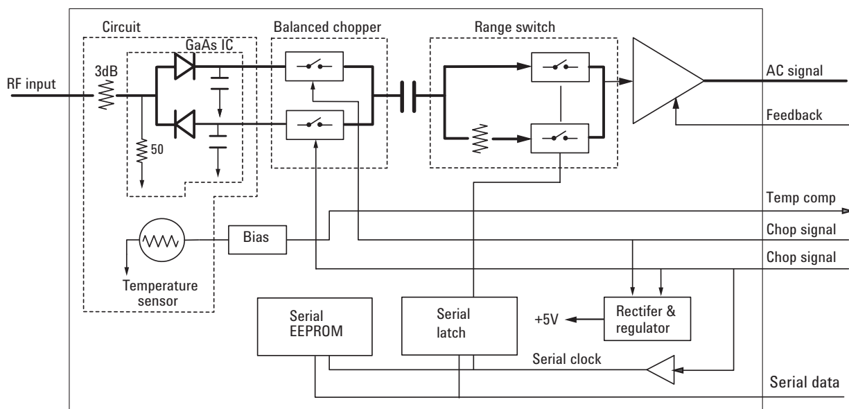
Figure 6. The power sensor's EEPROM stores linearity, temperature compensation, and calibration factor corrections that are used to achieve a 90 dB power range.
