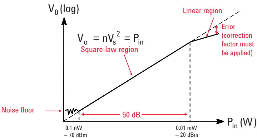
Figure 5. Diode detection ranges from the square law region to a linear region, where correction factors are applied.
