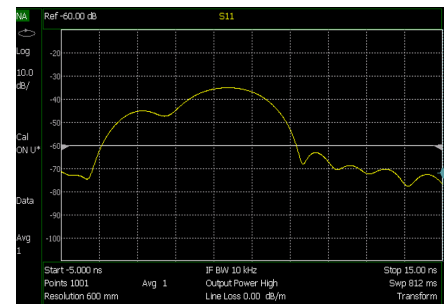
(a) Time response with 500 MHz span
