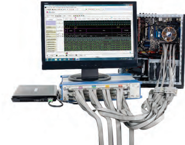
Figure 6. U4154A-4 Gb/s DDR3 logic analyzer solution
