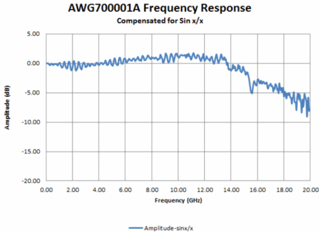
Figure 13. AWG70001 frequency response after removing the influence of the DAC's \text{Sinc}(f) response. The low attenuation of frequencies as high as 20 GHz permits the direct generation of modulated carriers at those frequencies.
