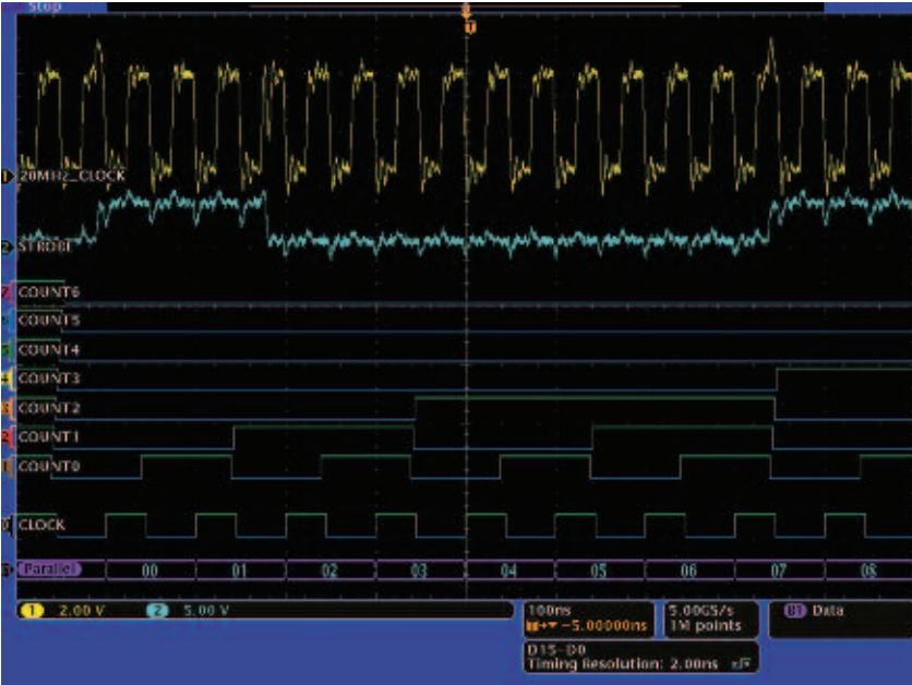
Visualize digital signal operation with time correlated views of both digital and analog information on a Mixed Signal Oscilloscope
