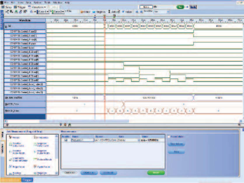
Instantly move probe points without recompiling your design and correlate internal FPGA signal activity to board-level signals
