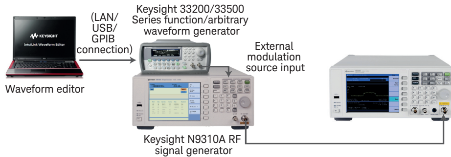
Figure 3. Equipment configuration for FSK signal generation and measurement
