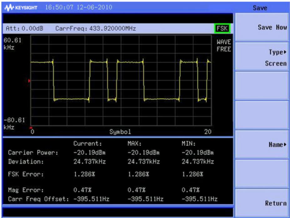
Figure 11. FSK demodulation – waveform view
