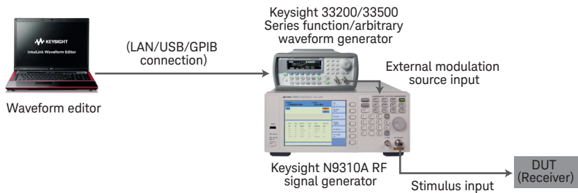
Figure 1. A typical system setup for measuring ASK/FSK receivers
