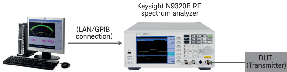
Figure 2. A typical system setup for measuring ASK/FSK transmitters
