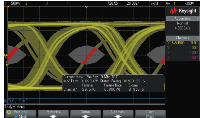
Figure 5: FlexRay eye-diagram mask test shows significant physical layer issues when probed at the input of a particular FlexRay receiver.
