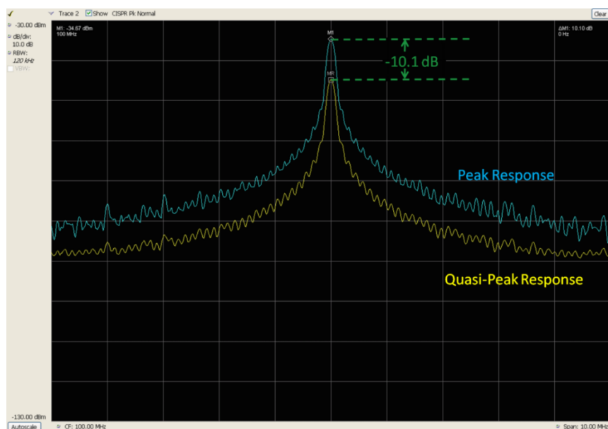
Figure 5. Peak Response vs Quasi-Peak Response 5: Peak Response vs Quasi-Peak Response
