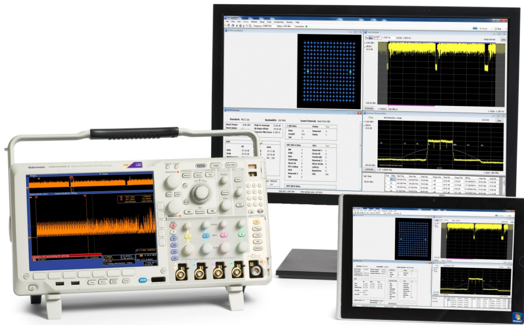
Figure 15. Tektronix MDO4000B Paired with SignalVu-PC to Analyze 802.11ac Signals
