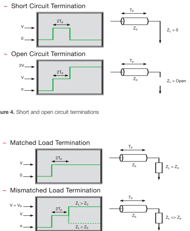
Figure 5. Matched and mismatched load terminations
