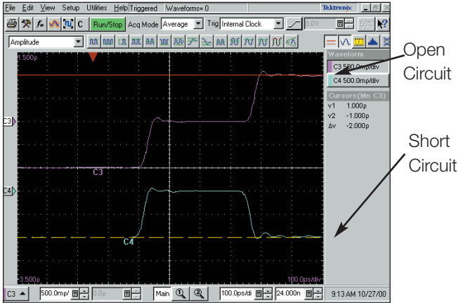
Figure 2. Time domain measurement shows a step with an open and a short circuit. The short circuit is measured as -1\text{ p (rho)} and the open circuit (infinite ohms) results in a \rho of +1 .
