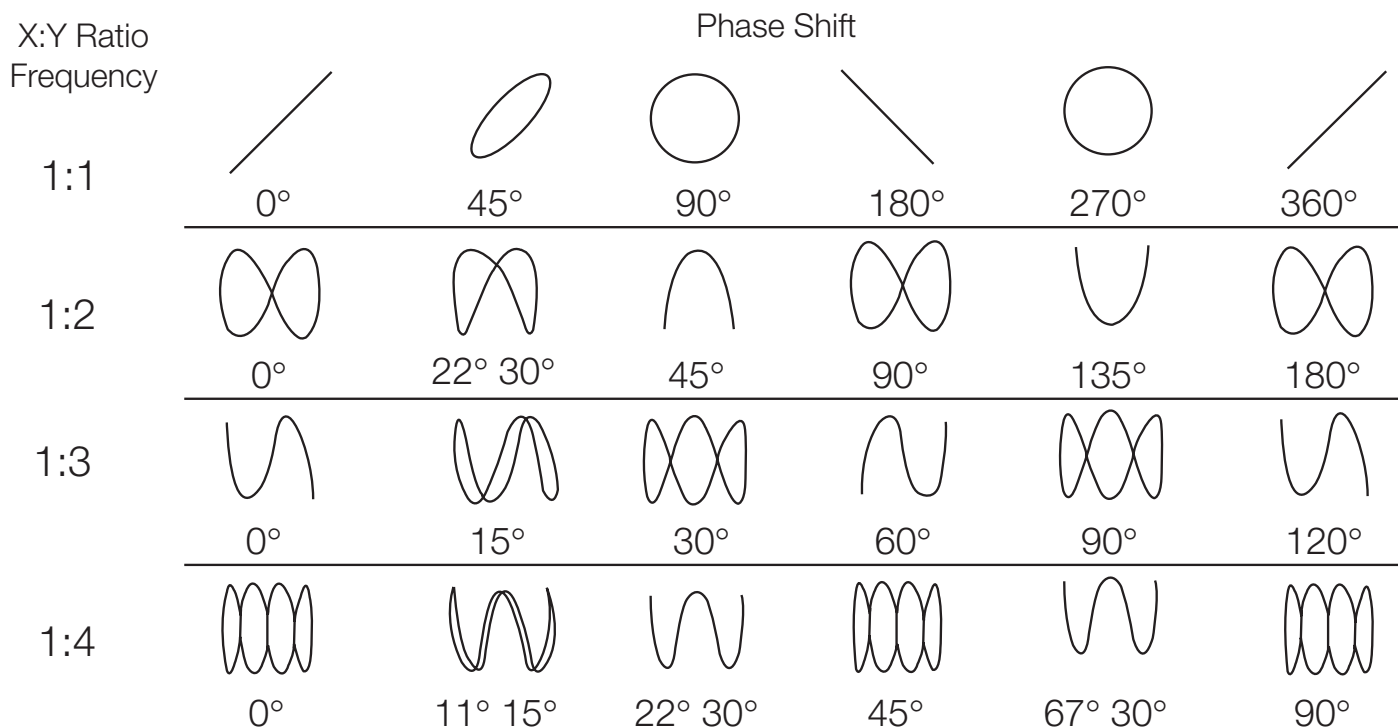
Figure 70. Lissajous patterns.
