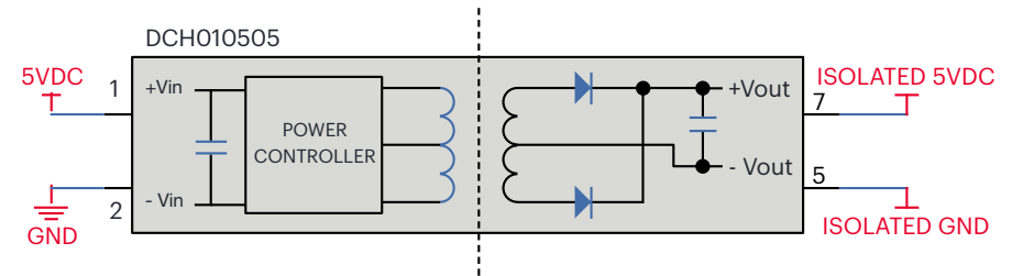
Figure 10. Isolated input circuit diagram
