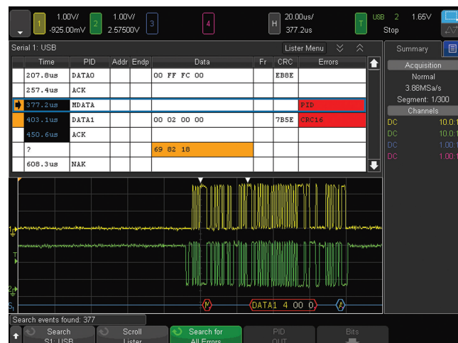
Figure 21. USB 2.0 trigger, decode and "lister" display.
